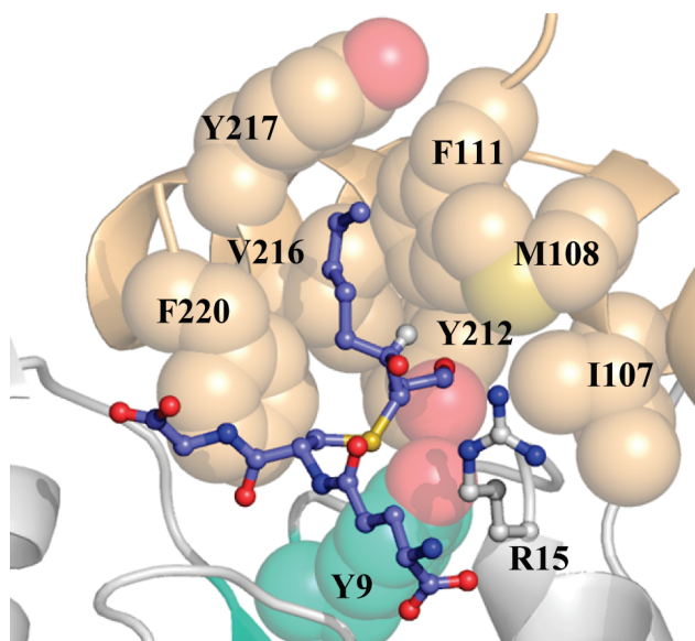
FIGURE 4: Human GSTA4-4 active site. GSTA4-4 is shown in complex with 3 S ,4 R -GSDHN (PDB entry 3IK7, blue ligand). The conserved G-site is toward the bottom half of the figure, with Y9 colored cyan. The 4-hydroxyl group is orientated toward R15, while the aldehyde-derived hydroxyl is in the proximity of Y212 at the bottom of the H-site. Other important active site residues are labeled and shown as spheres to illustrate the hydrophobic cavity.
