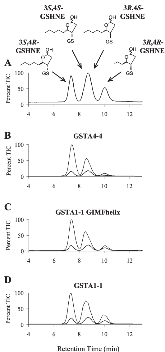
FIGURE 2: Comparison of stereoselectivity of product formation. The GSHNE diastereomers were prepared by incubation of GSH and (A) buffer alone, (B) GSTA4-4, (C) GSTA1-1 GIMFhelix, or (D) GSTA1-1, with racemic HNE, and analyzed by LC-MS (ESI+, m/z 464). The corresponding spontaneous reaction (gray line) is also shown for the sake of comparison.
