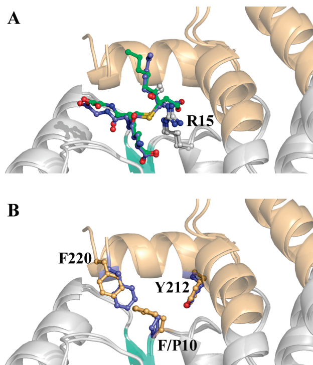
FIGURE 5: Position of residues 10 and 220 within human A-class GST active sites. (A) Structural superposition of 3 S ,4 R -GSDHN-bound GSTA4-4 (PDB entry 3IK7, blue ligand) and 3 S ,4 R -GSDHN-bound GSTA1-1 GIMFhelix (PDB entry 3IK9, green ligand). (B) Structural superposition contrasting the side chain of F/P10 and F220. The ball-and-stick representations of residues from the GSTA4-4 and GSTA1-1-GIMFhelix complexes are colored blue and orange, respectively. The ligands are not shown for the sake of clarity in panel B.
