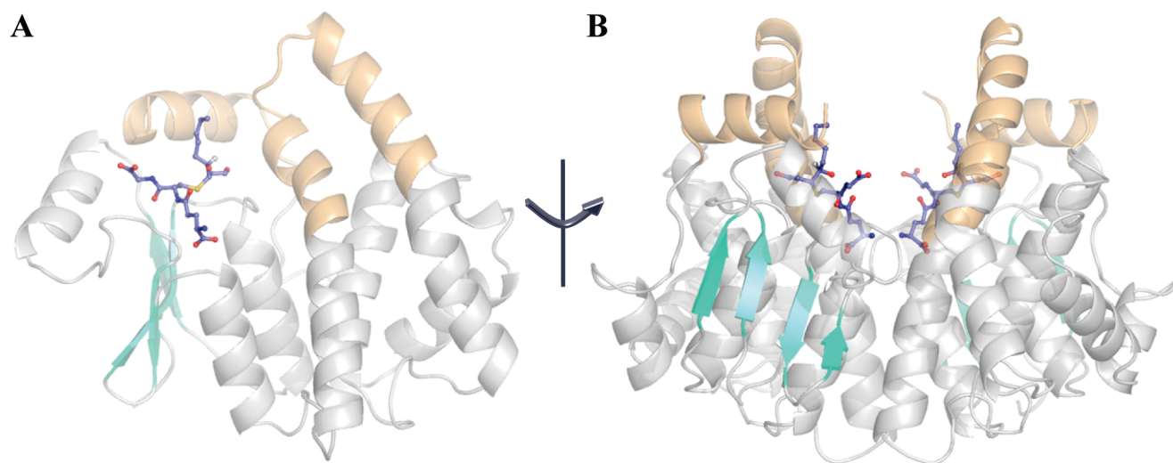
FIGURE 3: Overall structure of human GSTA4-4 in complex with 3S,4R-GSDHN (PDB entry 3IK7). The views are aligned perpendicular to the 2-fold axis of symmetry for the dimer. (A) Structure emphasizing the active site region within one subunit ( \beta -strands colored cyan, \alpha -helices colored gray, except for the C-terminal and \alpha 4 – \alpha 5 tower regions, which are highlighted in orange throughout all figures). (B) Semitransparent view of the dimer.
