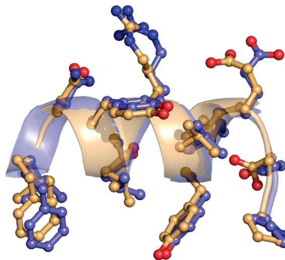
FIGURE 6: C-Terminal regions of apo and ligand-bound human GSTA4-4. Structural superposition of apo (PDB entry 1GUM, orange) and 3S,4R-GSDHN-bound GSTA4-4 (PDB entry 3IK7, blue) illustrating the localized structure of helix \alpha 9 regardless of ligand occupancy. Only residues 208–220 are shown for the sake of clarity.
