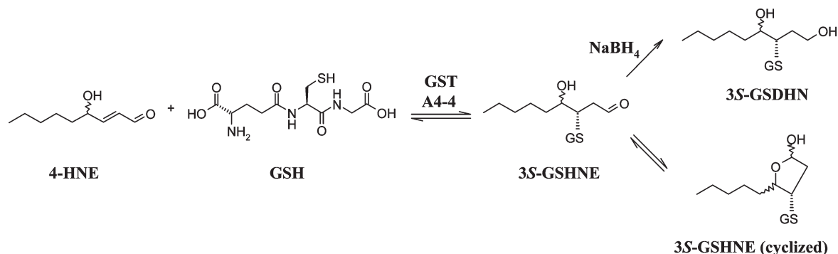
FIGURE 1: Reaction of racemic HNE with GSH. 1,4-Addition reaction of HNE with GSH as catalyzed by human GSTA4-4, followed by intramolecular cyclization or reduction by NaBH 4 .
